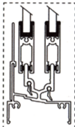
Alternative Cill Rail with extended Water leg
