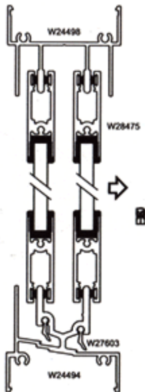
Alternative Cill Rail with extended Water leg
